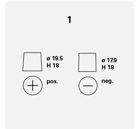
Terminal Tipleri
